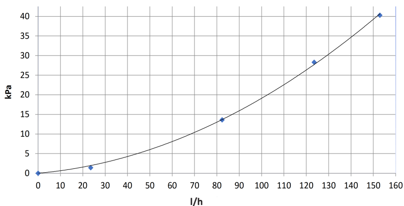
TS 300 Graph: Pressure Drop (kPa) vs Flow Rate (l/h) Medium: Thesol (Propylene glycol 50%) Temperature: 50 °C
